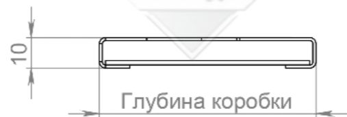
Порог без притвора 15, 20, 25, 30, 35, 40, 45, 50, 55, 60
